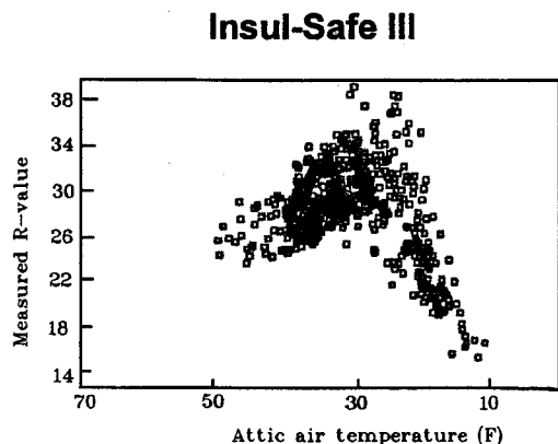
Figure 1 — Measured R-value of nominal R-34 loose-fill fiberglass attic insulation at various attic air temperatures. Tests were performed at the University of Illinois.
